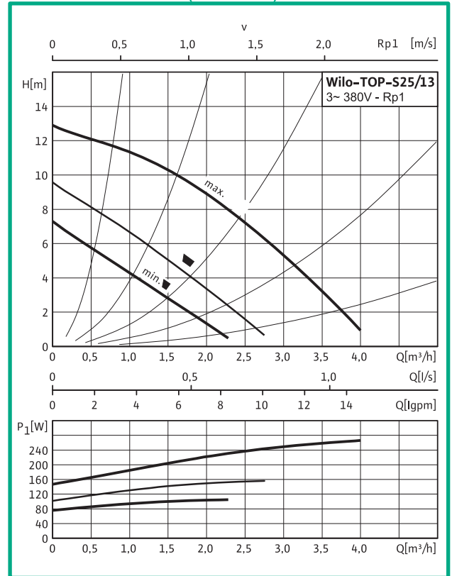
TOP-S 25/13 DM (3~380V)
