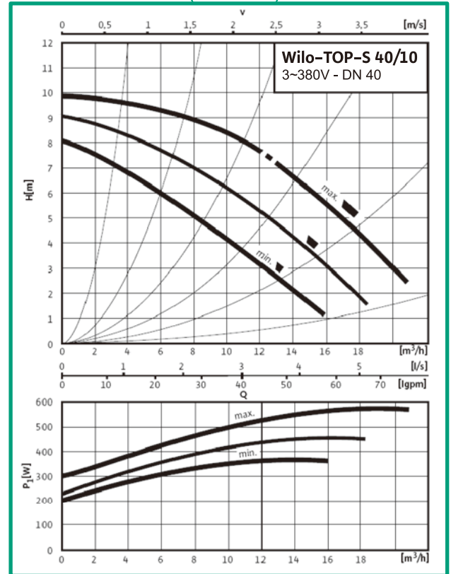
TOP-S 40/10 DM (3~380V)
