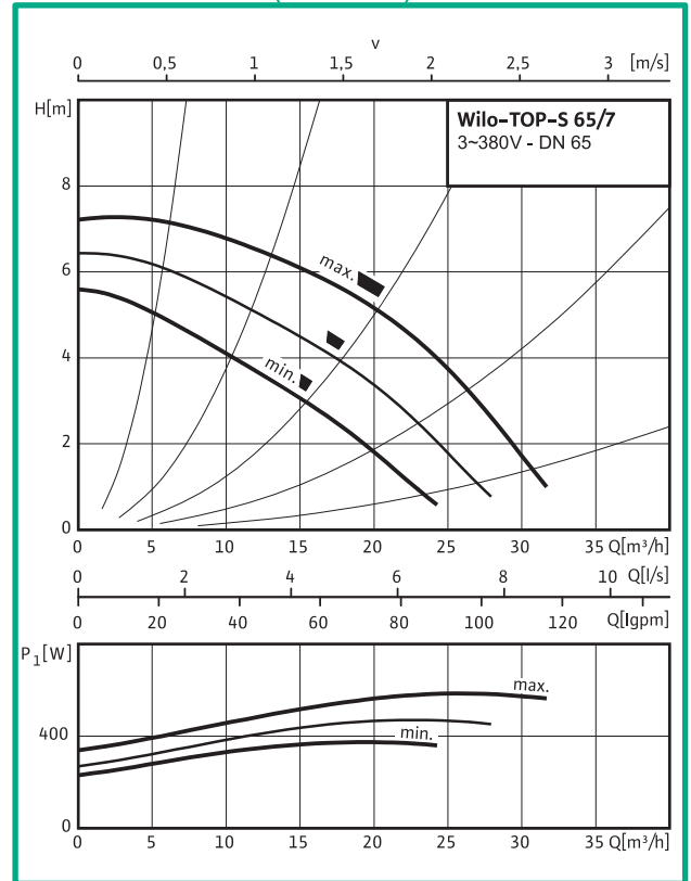
TOP-S 65/7 DM (3~380V)
