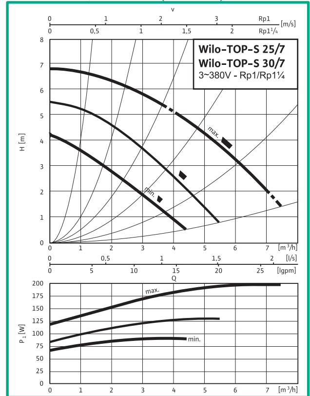
TOP-S 25/7, 30/7 DM (3~380V)
