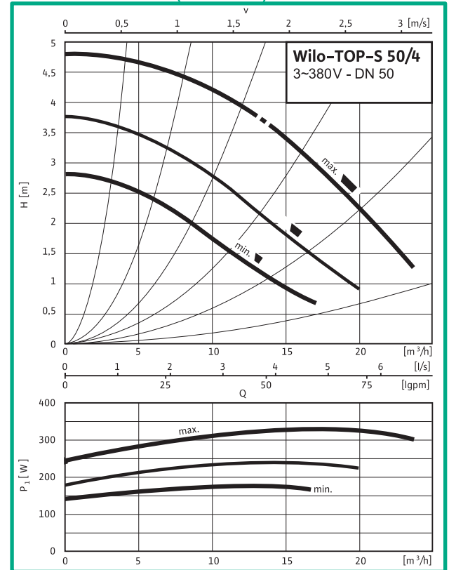
TOP-S 50/4 DM (3~380V)
