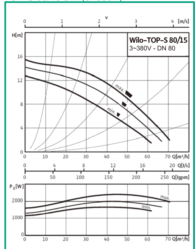
TOP-S 80/15 DM (3~380V)
