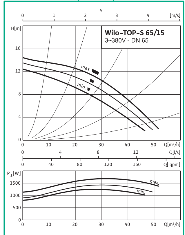
TOP-S 65/15 DM (3~380V)
