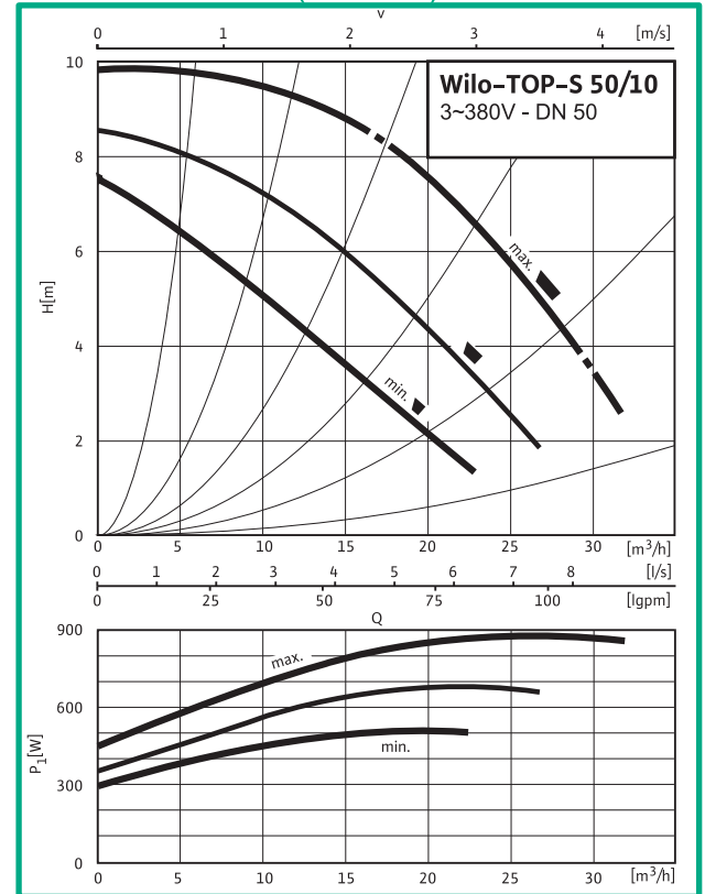
TOP-S 50/10 DM (3~380V)
