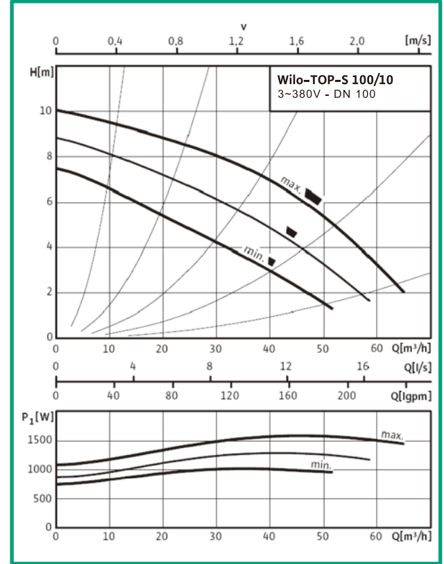
TOP-S 100/10 DM (3~380V)
